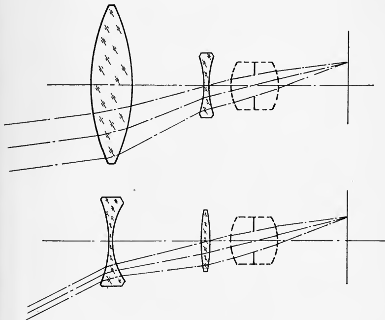
FIG. 7. Telephoto and wide angle attachments.
